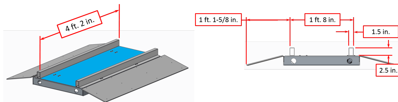
Figure 2-9: Moat Dimensions
