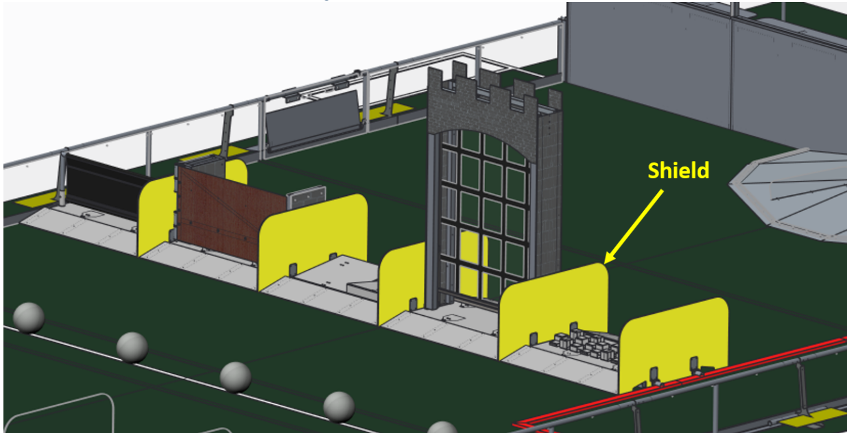
Figure 2-20: Shield Locations
